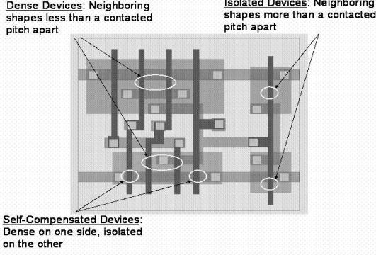
Figure 5: An example cell layout depicting isolated, dense and self-compensated devices.
