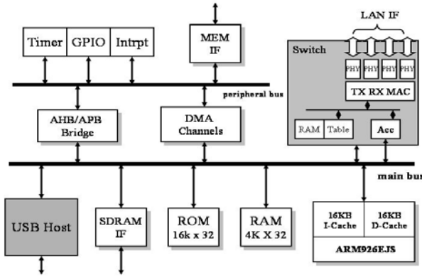
Figure 4. SoC platform
