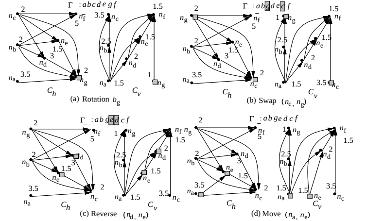
Figure 4: Four types of perturbation. (a) The resulting TCG-S after rotating the module b_g shown in Figure 2(b). (b) The resulting TCG-S after swapping the nodes n_c and n_g shown in (a). (c) The resulting TCG-S after reversing the reduction edge (n_d, n_e) shown in (b). (d) The resulting TCG-S after moving the reduction edge (n_a, n_e) from the C_v of (c) to C_h .
