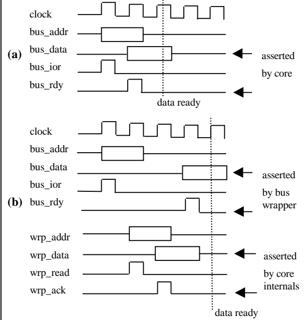
Figure 5 : Timing diagrams for a custom peripheral bus: (a) Read cycle of an integrated core, (b) read cycle of a core with a wrapper (Non-PVCI or PVCI).
