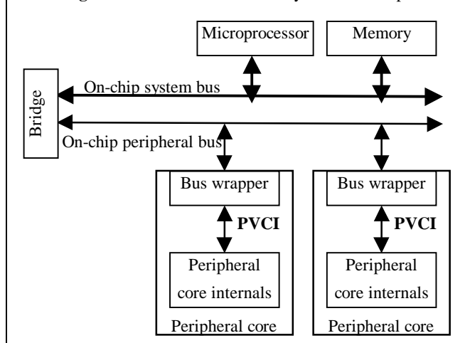
Figure 1 : PPCI's location in a system-on-a-chip.
