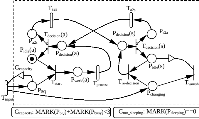
Figure 2 Example GSPN model of a USS.
