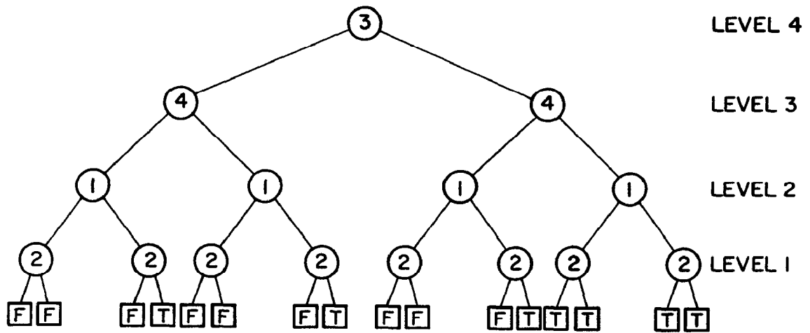
FIG. 1 A BINARY DECISION TREE REPRESENTING f(x_1, x_2, x_3, x_4) = x_1 x_2 + x_3 x_4
