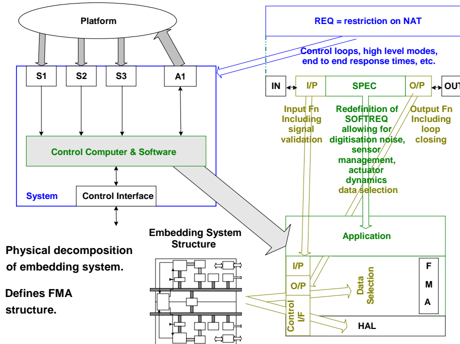
Fig. 2. Representation of Software Structure
