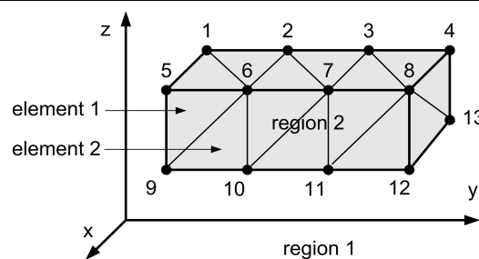
Figure 3. Mesh format.
