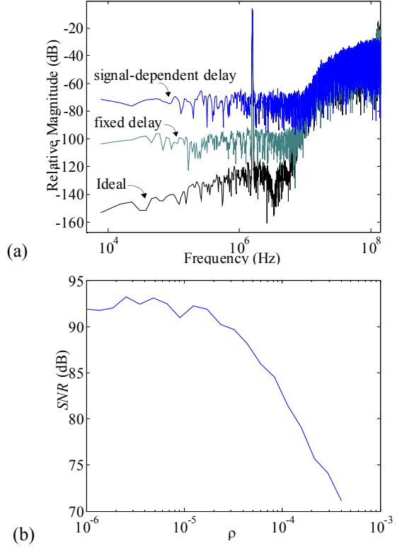
Fig. 8: Effect of (a) loop delay time and (b) clock jitter noise on CT 5th-LP ΣΔM.
