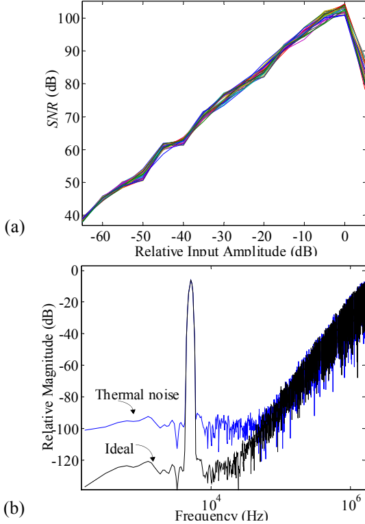
Fig. 7: Effect of (a) mismatch error and (b) thermal noise on SC 2-1 sb ΣΔM.
