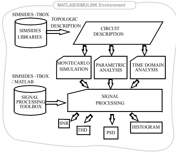
Fig. 3: Structure of SIMSIDES.
