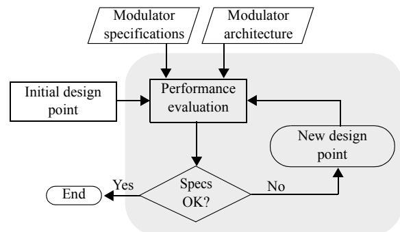
Fig. 1: Conceptual block diagram of an optimization-based \Sigma\Delta synthesis tool.
