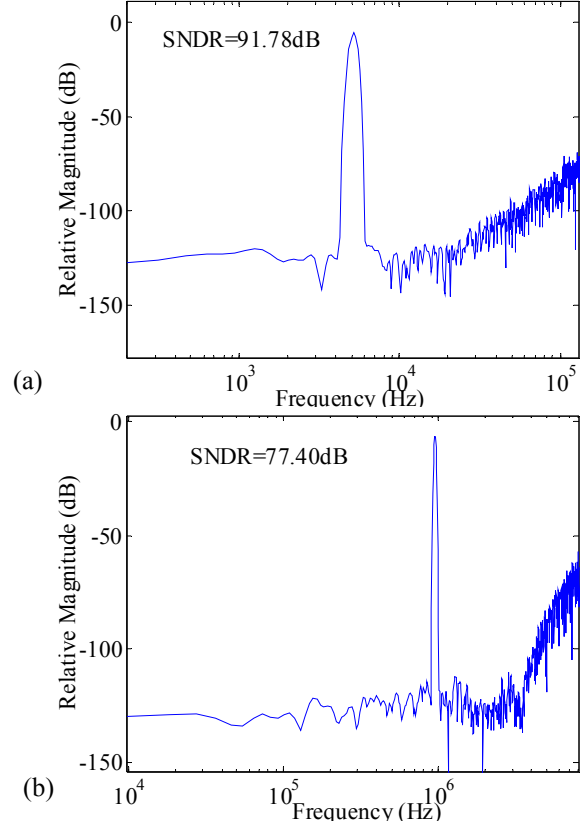
Fig. 9: Output spectra and SNDR of the synthesized (a) SC 2-1 sb and (b) CT 5th-order LP \Sigma\Delta Ms.
