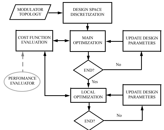
Fig. 2: Operation flow of the optimization core.
