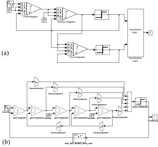
Fig. 6: Block diagrams of the (a) SC 2-1 sb ΣΔM and (b) CT 5th-order LP ΣΔM.
