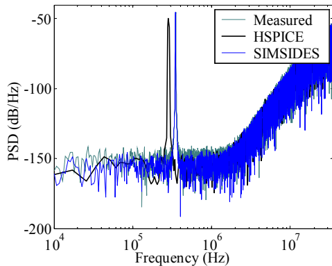
Fig. 4: Simulation of a SC cascade 2-1-1.
