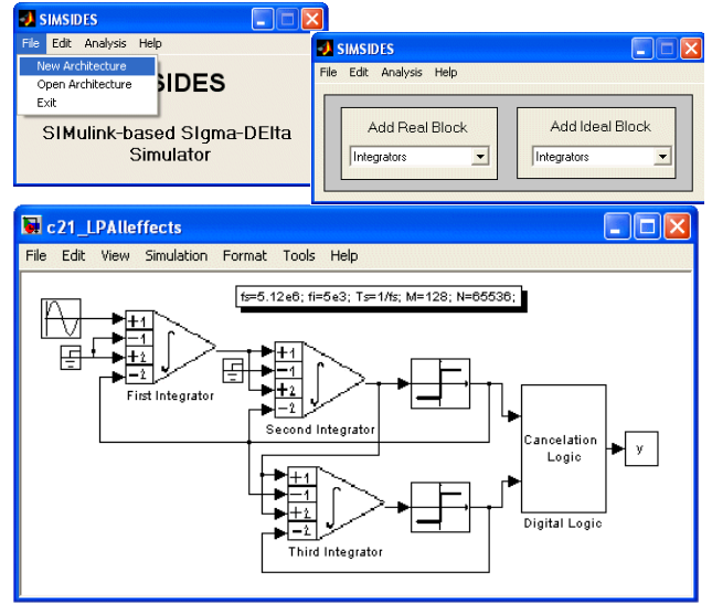
Fig. 5: Illustrating the GUI for editing modulator topologies of the \Sigma\Delta Synthesis Toolbox.
