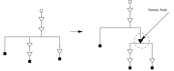
Figure 5: Transformation of Non binary tree to Binary Tree
