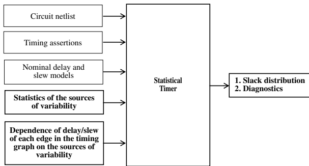
Figure 1: Block diagram of a statistical timer.
