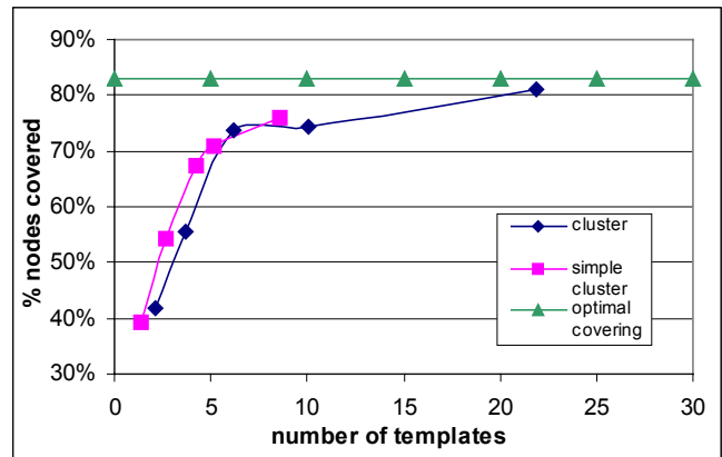
Figure 3 Comparison of clustering techniques
