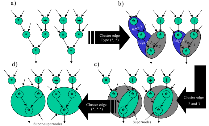
Figure 2 Contraction of edges to create supernodes. The supernodes correspond to templates.
