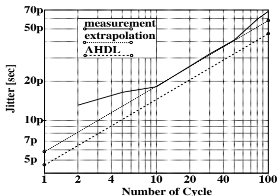
Figure 4: Jitter at N' th cycle
