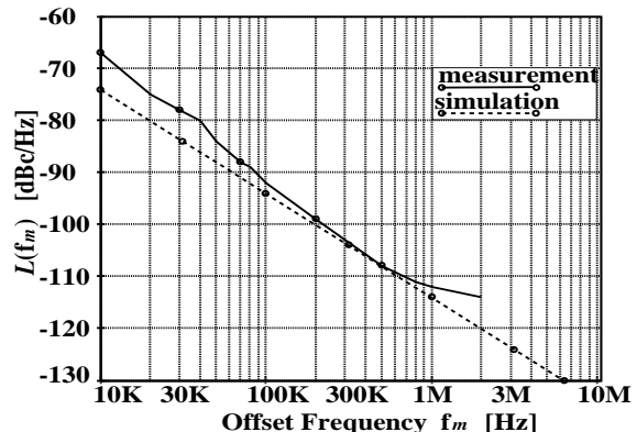
Figure 3: Phase noise vs. offset frequency.
