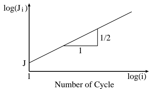
Figure 2: Jitter in the length of i adjacent cycles.
