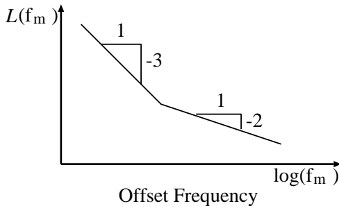
Figure 1: L(f_m) vs. offset frequency
