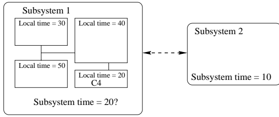
Fig. 3: Subsystem_1 must stall to maintain continuous consistency.
