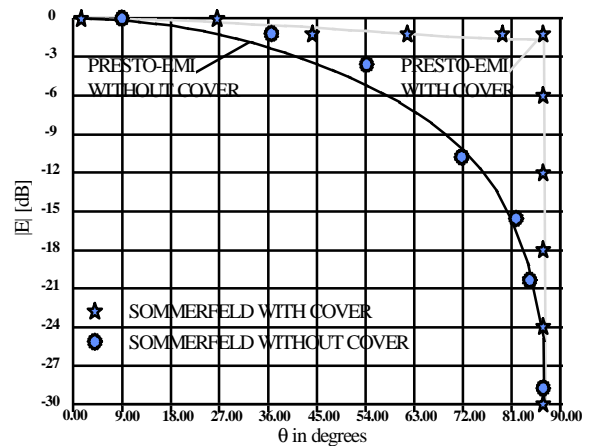
Figure 8(b): E-plane pattern for the (embedded) microstrip
