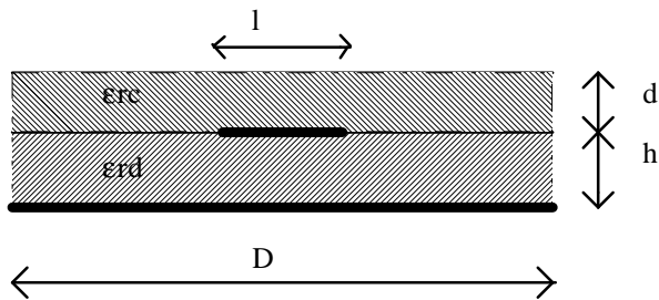
Figure 7: embedded microstrip
