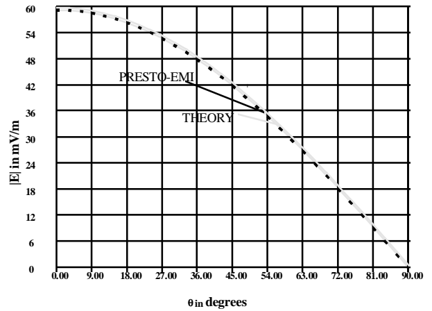
Figure 4(b): H-plane pattern for an Hertzian dipole above a metal plane (h = 1 cm)
