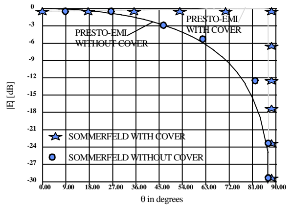
Figure 8(a): H-plane pattern for the (embedded) microstrip
