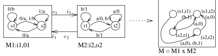
Figure 2: Forming the Product Machine
