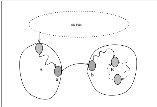
Figure 4: Adding edge ab can potentially add all states in A and B to Fair^+
