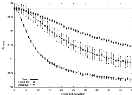
Fig. 2. Effect of noise on the average (real) fitness of individuals selected by pairwise tournament selection. The adaptive method remains closer to the expected fitness than the fixed-size sampling.
