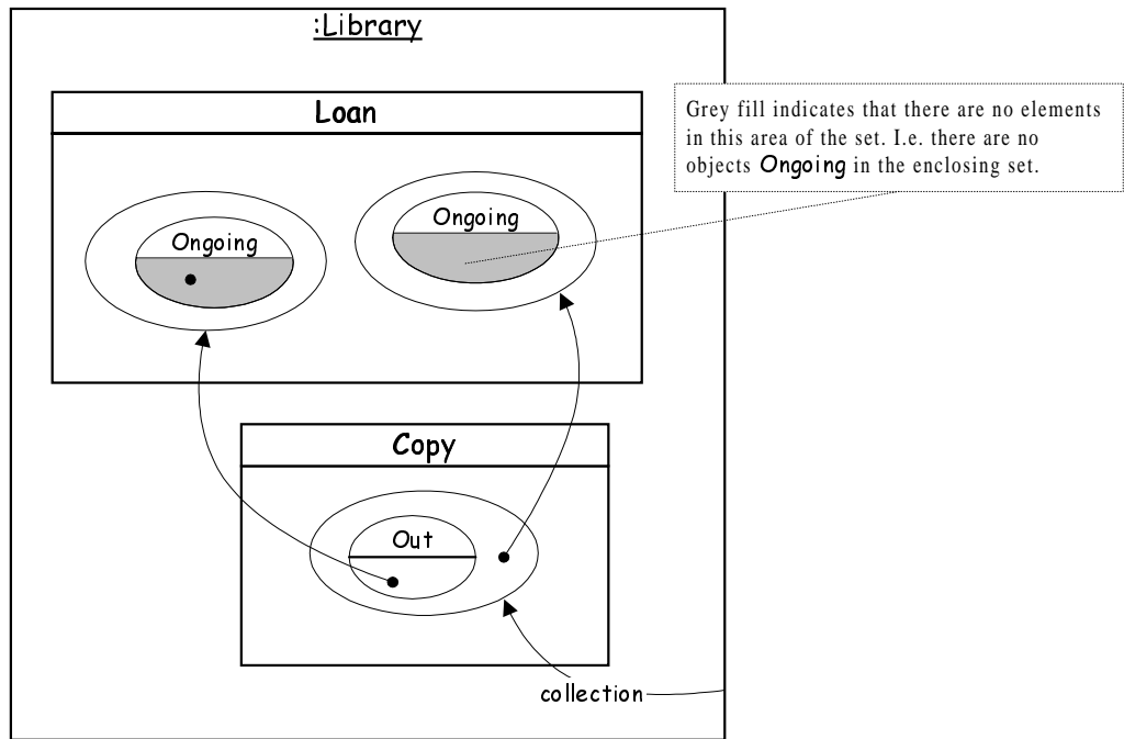
Figure 11: Constraint diagram for invariant 4
