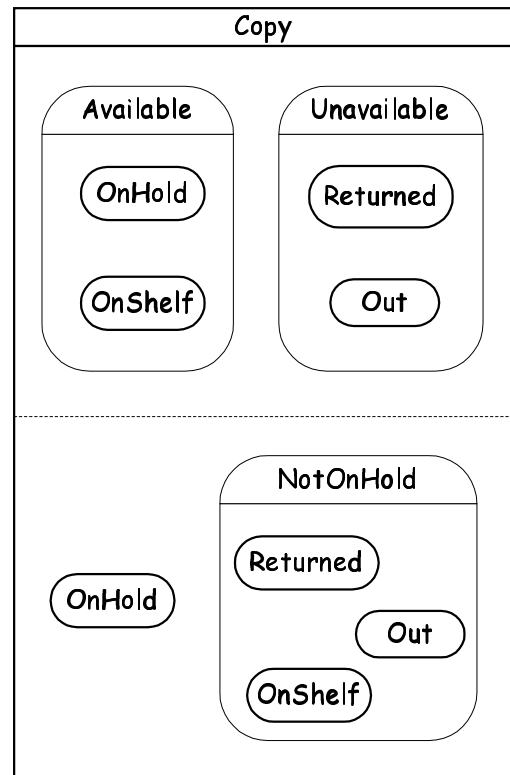
Figure 16: A possible state diagram for Copy (transitions omitted)
