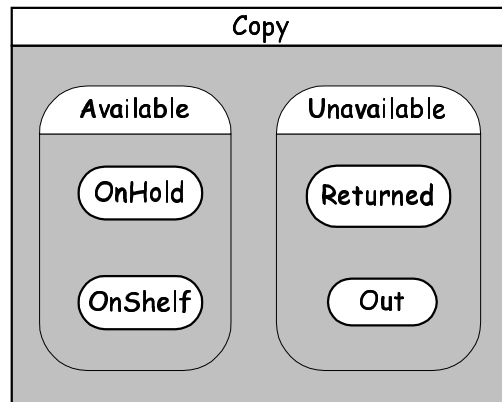
Figure 13: A grouping of states for Copy
