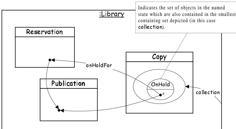
Figure 8: Constraint diagram for invariant 1
