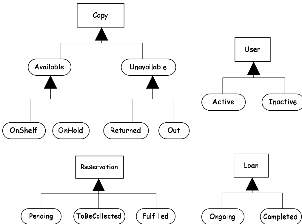
Figure 3: Type diagrams showing states
